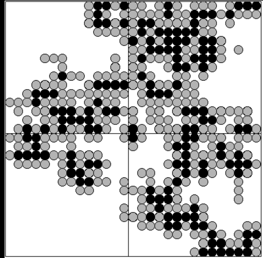
Perkolationsimulering
