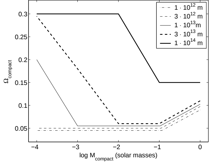
Fig. 5. Same as Fig. 2 for the z > 1.5 part of the VAR sample of H2000.
