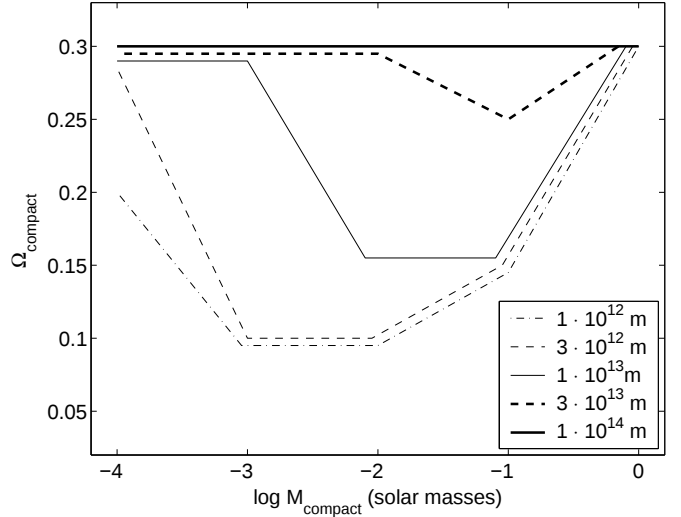
Fig. 3. Same as Fig. 2 for the UVX sample of H2000.
