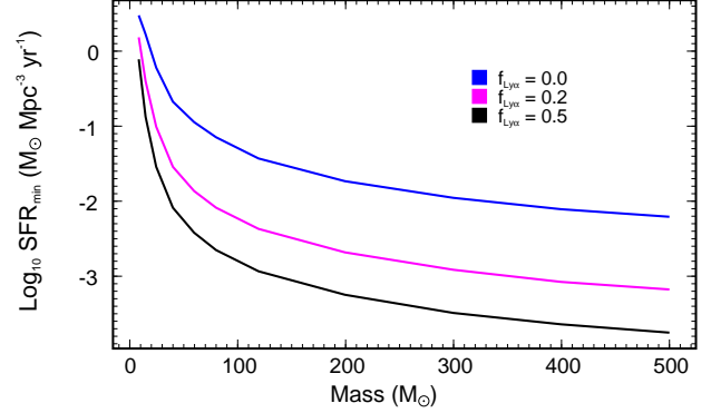
Figure 5. The \text{SFR}_{\min} in the MACS J0717.5+3745 field, as a function of the population III mass (assuming all such stars to have the same mass) at z = 15 . Imaging in the NIRCam /F200W filter is assumed. Since this graph uses a single filter, it is not necessarily the filter resulting in the lowest \text{SFR}_{\min} . This means that the values in this graph differ in some instances from the values in Figure 3 and 4, where the filter resulting in the lowest \text{SFR}_{\min} is always selected. The detection criterion is based on a 10\sigma detection after an exposure time of 100h. The blue line represents the \text{SFR}_{\min} with no \text{Ly}\alpha radiation escaping, whereas the purple and black lines represent f_{\text{Ly}\alpha} = 0.2 and 0.5 , respectively. A higher population III stellar mass results in a lower required SFR. This indicates that a top heavy IMF improves the prospects of detecting high-redshift population III stars.
