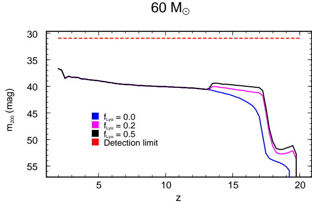
Figure 1. The NIRCcam/F200W AB magnitude predicted for a 60 M_{\odot} star as a function of redshift in an unlensed field. The blue line represents the magnitude with no \text{Ly}\alpha radiation escaping, whereas the purple and black lines represent f_{\text{Ly}\alpha} = 0.2 and 0.5 , respectively. The red dashed line indicates the detection limit (30.9 mag) considering S/N = 10 , using an exposure time of 100h. As seen, the unlensed flux of a 60 M_{\odot} population III star lies \gtrsim 6 magnitudes below the JWST detection threshold.
