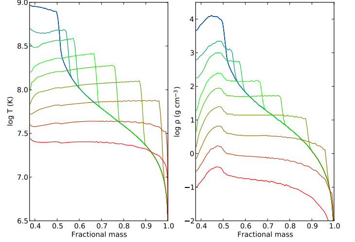
Fig. 5. Evolution of the temperature (left panel) and density (right panel) profiles between 1 and 282 seconds (shock breakout) in 10 logarithmically spaced intervals for the 4 M_{\odot} helium-core model, where the time has been colour coded from blue (early) to red (late).
