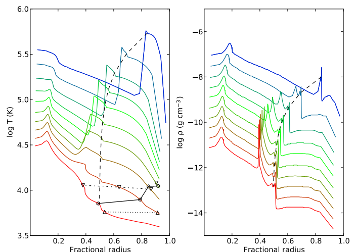
Fig. 10. Evolution of the temperature (left panel) and density (right panel) profiles between shock breakout (0.3 days) and the luminosity minimum (11 days) in 10 logarithmically spaced intervals for the 4.05 M_{\odot} MESA model, where the time has been colour coded from blue (early) to red (late). The interface between the helium and hydrogen envelopes (dashed line), the photosphere (circles and dashed line) and the helium (downward triangles and dot-dashed line) and hydrogen (upward triangles and dotted line) recombination fronts are also shown.
