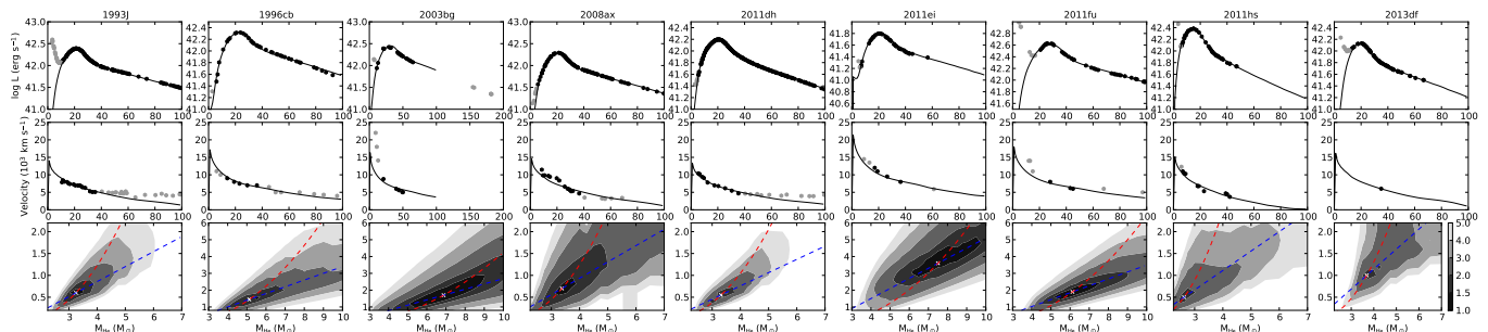
Fig. 12. Bolometric lightcurve (upper panels) and photospheric velocity evolution (middle panels) for the best-fit models as compared to the observed UV to MIR pseudo-bolometric lightcurve and estimated photospheric velocity evolution for the literature sample of Type IIb SNe. The lower panels show contour plots of the standard deviation in the fits, normalized to that of the optimal model, projected onto the E- M_{\text{He}} plane. We also show the constraints M_{\text{ej}}/E=\text{const} (blue) and M_{\text{ej}}^2/E=\text{const} (red) provided by the photospheric velocity evolution and the bolometric lightcurve, respectively.
