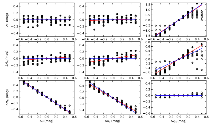
Fig. 13. Sensitivity of the derived explosion energy (upper panels), ejecta mass (middle panels), mass of ^{56}\text{Ni} (lower panels) to a change in the distance (left panels), extinction (middle panels) and photospheric velocities (right panels). For consistency the changes in all quantities are expressed in magnitudes. The derived quantities for the CSP and literature samples of Type IIb SNe are shown as black dots, power-law fits as red solid lines and the scalings expected from the Arnett (1982) model as blue solid lines.
