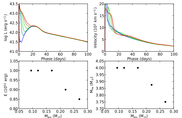
Fig. 9. Upper panels: Progression of model bolometric lightcurves (left panel) and photospheric velocities (right panel) calculated with HYDE for a 15 M_{\odot} MESA model with the mass-loss adjusted to yield a final mass of 4.2, 4.15, 4.1, 4.05, 4.025 and 4.0 M_{\odot} , colour coded from red ( 4.2 M_{\odot} ) to blue ( 4.0 M_{\odot} ). The SN parameters were E=1.0 \times 10^{51} \text{ erg} , M_{\text{Ni}}=0.1 M_{\odot} and \text{Mix}_{\text{Ni}}=M_{\text{He}}/M . Lower panels: Sensitivity of the explosion energy (left panel) and helium-core mass (right panel) to the mass of the hydrogen envelope, calculated by fitting the model lightcurves and photospheric velocities to the model grid using the procedure described in Sect. 5.2.
