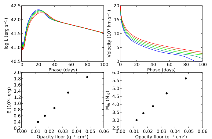
Fig. 8. Upper panels: Model bolometric lightcurves (left panel) and photospheric velocities (right panel) for day 1-100 showing the dependence on the opacity floor ( 0.012\text{-}0.048 \text{ g}^{-1} \text{ cm}^2 ). Low to high values are displayed in blue to red colour coding and the model parameters are M_{\text{He}}=4.0 M_{\odot} , E=1.0 \times 10^{51} erg, M_{\text{Ni}}=0.1 M_{\odot} and \text{Mix}_{\text{Ni}}=1.0 . Lower panels: Sensitivity of the explosion energy (left panel) and helium-core mass (right panel) to the opacity floor, calculated by fitting the model lightcurves and photospheric velocities to the model grid using the procedure described in Sect. 5.2.
