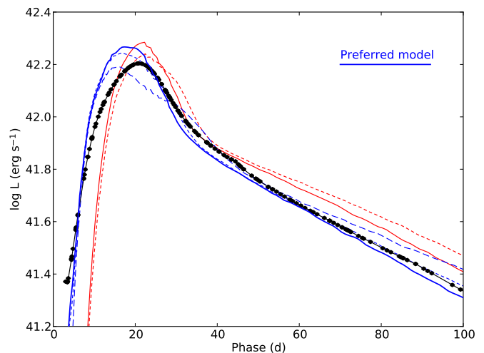
Fig. 18. The 3–100 days J14 model bolometric lightcurves calculated with HYDE, compared to the observed optical-to-MIR pseudo-bolometric lightcurve (black circles). The model families differing in initial mass ( 12 M_{\odot} ; solid, 13 M_{\odot} ; short-dashed, 17 M_{\odot} ; long-dashed) and macroscopic mixing (medium; red; strong; blue) are shown. Following this coding, the preferred model is shown as a blue solid line.
