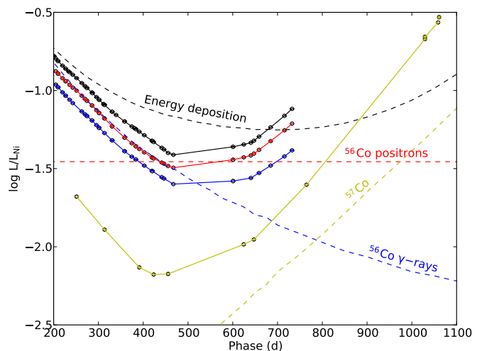
Fig. 23. The >200 days optical-to-MIR (black dots), optical-plus-MIR (red dots), optical and MIR (yellow dots) pseudo-bolometric lightcurves, as compared to the bolometric lightcurve (black dashed line), deposited ^{56}\text{Co} \gamma -ray (blue dashed line) and positron (red dashed line) luminosity and deposited ^{57}\text{Co} luminosity (yellow dashed line) for the preferred steady-state NLTE model (12F). The lightcurves have been normalized to the radioactive decay chain luminosity of 0.075 M_{\odot} of ^{56}\text{Ni} .
