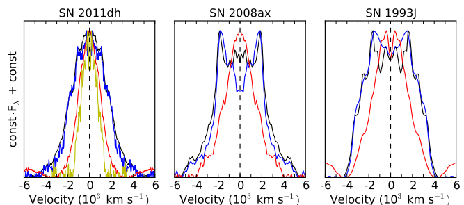
Fig. 12. Continuum subtracted mirrored blue-side profiles for the [\text{O I}] 6300 \text{\AA} (black), \text{Mg I}] 4571 \text{\AA} (blue), [\text{Ca II}] 7291 \text{\AA} (red) and [\text{Fe I}] 7155 \text{\AA} (yellow) lines for SNe 2011dh, 2008ax and 1993J at 300, 307 and 283 days respectively. The [\text{Fe I}] 7155 \text{\AA} line is only shown for SN 2011dh.
