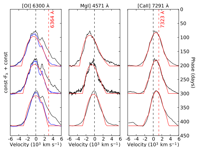
Fig. 11. The [\text{O I}] 6300,6364 \text{\AA} (left panel; black), decomposed [\text{O I}] 6300 \text{\AA} (left panel; blue), \text{Mg I}] 4571 \text{\AA} (middle panel; black) and [\text{Ca II}] 7291,7323 \text{\AA} (right panel; black) lines at selected epochs, as compared to line profile fits (red). The [\text{O I}] 6300 \text{\AA} line was decomposed with the method described in Appendix B.
