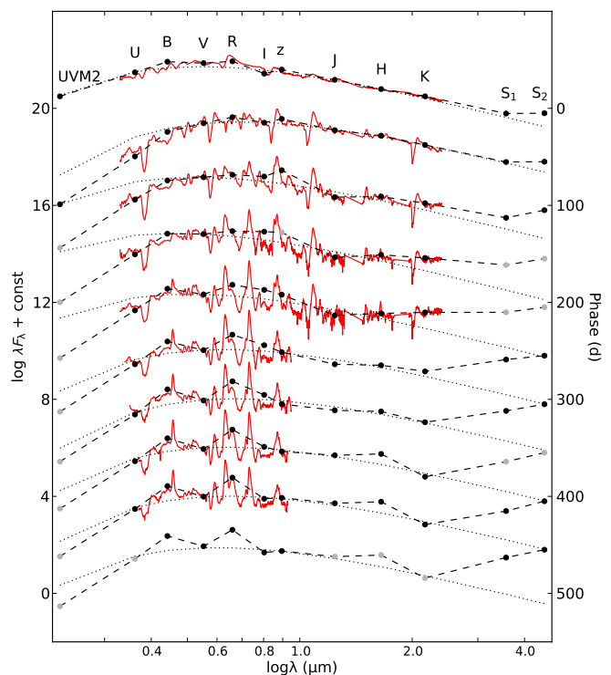
Fig. 6. The <500 days evolution of the SED (black dots and dashed lines), overplotted with blackbody fits to the V , I , J , H and K photometry (black dotted lines) as well as the observed (interpolated; Sect. 3.1) spectra (red solid lines). Fluxes based on extrapolations or >25 days interpolations are displayed in shaded colour.
