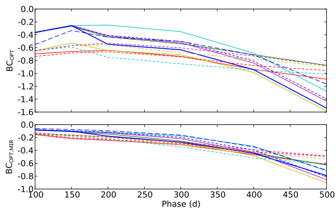
Fig. C.1. 100–500 days optical (upper panel) and optical-to-MIR (lower panel) BCs for the J14 models. The models are displayed as in Fig. 17.
