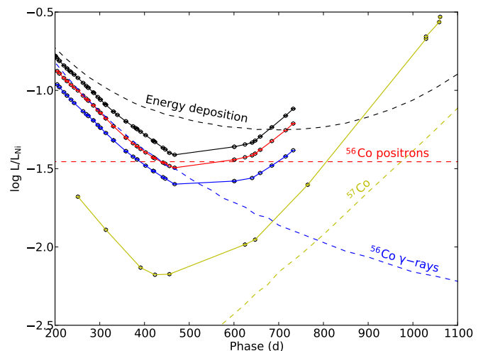
Fig. 23. The >200 days optical-to-MIR (black dots), optical-plus-MIR (red dots), optical (blue dots) and MIR (yellow dots) pseudo-bolometric lightcurves, as compared to the bolometric lightcurve (black dashed line), deposited ^{56}\text{Co} \gamma -ray (blue dashed line) and positron (red dashed line) luminosity and deposited ^{57}\text{Co} luminosity (yellow dashed line) for the preferred steady-state NLTE model (12F). The lightcurves have been normalized to the radioactive decay chain luminosity of 0.075 M_{\odot} of ^{56}\text{Ni} .
