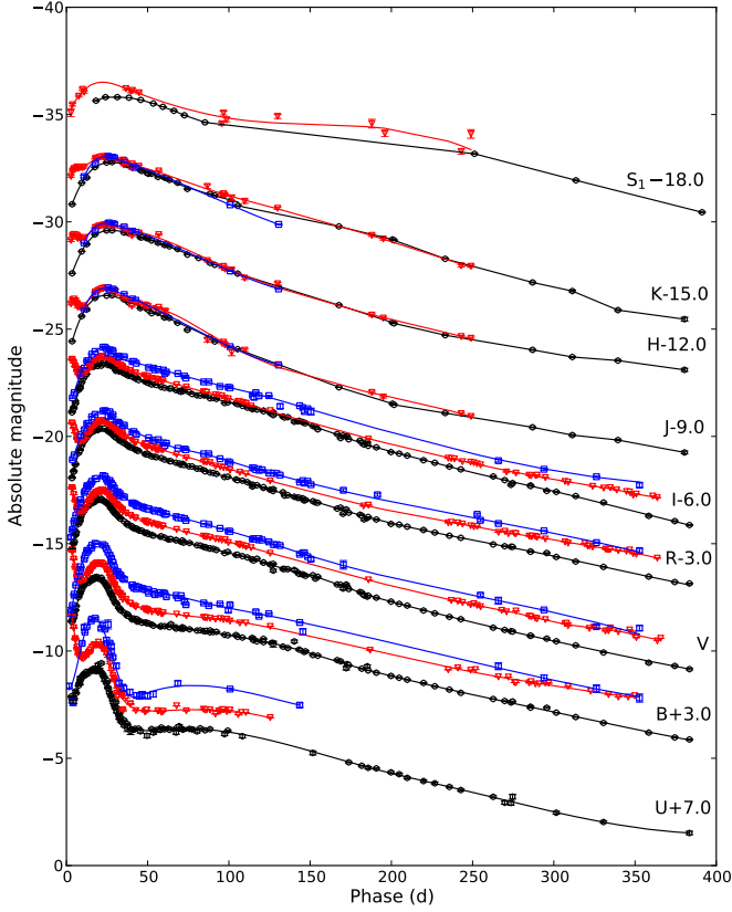
Fig. 2. The <400 days absolute optical, NIR and MIR broad-band lightcurves for SNe 2011dh (black circles), 1993J (red triangles) and 2008ax (blue squares). For clarity each band has been shifted in magnitude. Each lightcurve has been annotated with the name of the band and the shift applied. We also show combinations of spline fits, interpolations and extrapolations used in calculations.
