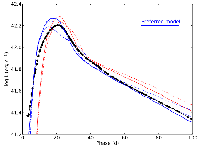
Fig. 18. The 3–100 days J14 model bolometric lightcurves calculated with HYDE, as compared to the observed optical-to-MIR pseudo-bolometric lightcurve (black circles). The model families differing in initial mass ( 12 M_{\odot} ; solid, 13 M_{\odot} ; short-dashed, 17 M_{\odot} ; long-dashed) and macroscopic mixing (medium; red; strong; blue) are shown. Following this coding, the preferred model is displayed as a blue solid line.
