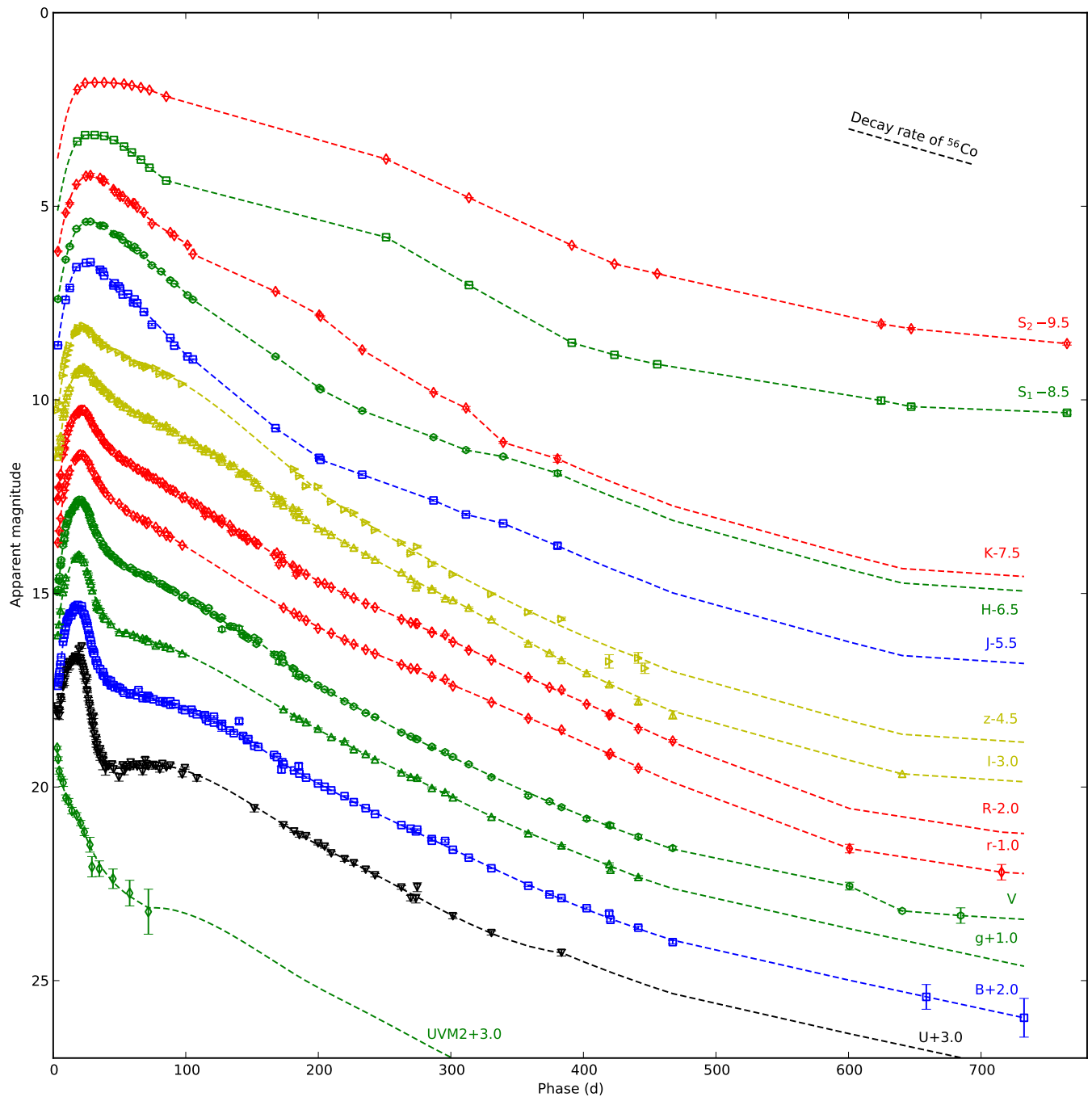
Fig. 1. The <800 days apparent UV, optical, NIR and MIR broad-band lightcurves for SN 2011dh. For clarity each band has been shifted in magnitude. Each lightcurve has been annotated with the name of the band and the shift applied. We also show combinations of spline fits, interpolations and extrapolations used in calculations.
