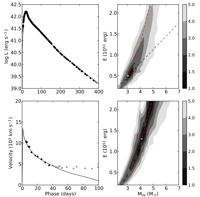
Fig. 22. Left panels: Optical-to-MIR pseudo-bolometric lightcurve (upper left panel) and photospheric velocities (lower left panel) for the best-fit model as compared to observations, where the photospheric velocities have been estimated from the absorption minimum of the Fe II 5169 Å line. Observations not included in the fit are displayed in grey. Right panels: Contour plots showing the (grey-scale coded) standard deviation in the fit, normalized to that of the best-fit model, projected onto the E - M_{\text{He}} plane for the case where the photospheric velocities were used (upper right panel) and not used (lower right panel). We also show the constraints M_{\text{ej}}/E=\text{const} (blue) and M_{\text{ej}}^2/E=\text{const} (red) provided by the photospheric velocities and the bolometric lightcurve, respectively (E15).
