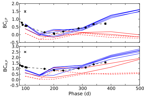
Fig. 19. The 100–500 days observed (black circles) and J14 model pseudo-BCs for the J and H -band. The model families differing in contrast factor (high; solid, low; short-dashed) and positron trapping (local; blue, non-local; red) are shown. 17 M_{\odot} and medium mixing models are not displayed. The error bars arising from the extinction are marked in the upper left or right corner.
