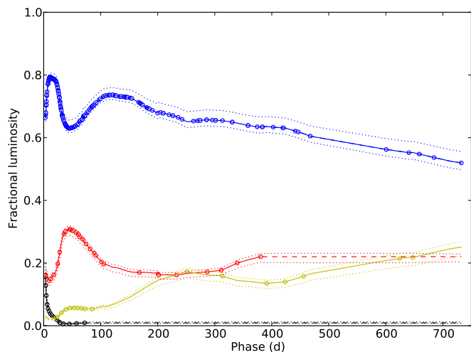
Fig. 5. The <750 days fractional UV (black dots), optical (blue dots), NIR (red dots) and MIR (yellow dots) luminosity for SN 2011dh. Interpolations and extrapolations are displayed as solid and dashed lines, respectively. The upper and lower error bars for the systematic error arising from extinction (dotted lines) are also shown.
