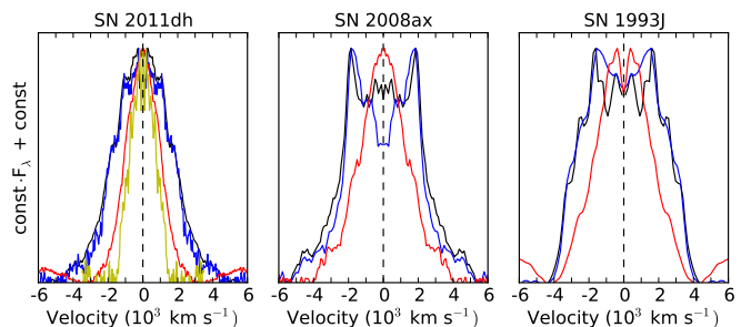
Fig. 12. Continuum subtracted mirrored blue-side profiles for the [O I] 6300 Å (black), Mg I 4571 Å (blue), [Ca II] 7291 Å (red) and [Fe I] 7155 Å (yellow) lines for SNe 2011dh, 2008ax and 1993J at 300, 307 and 283 days respectively. The [Fe I] 7155 Å line is only shown for SN 2011dh.
