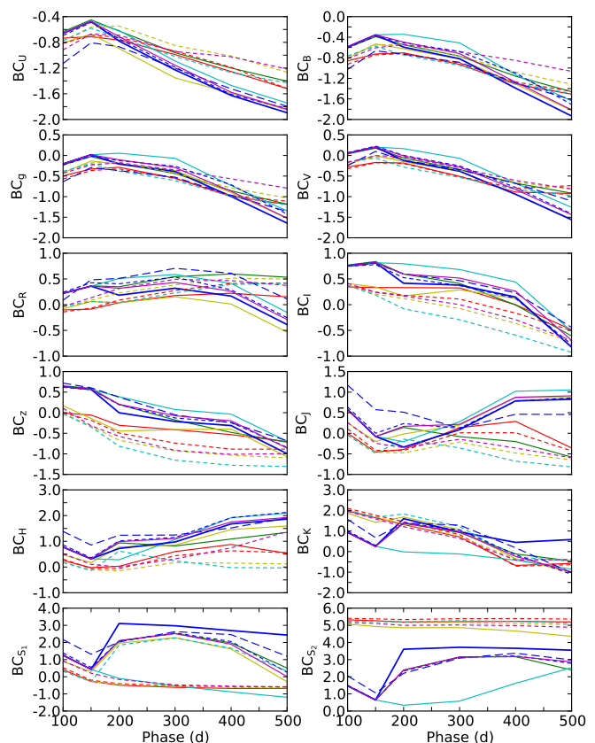
Fig. C.2. 100–500 days broad-band BCs for the J14 models. The models are displayed as in Fig. 17.
