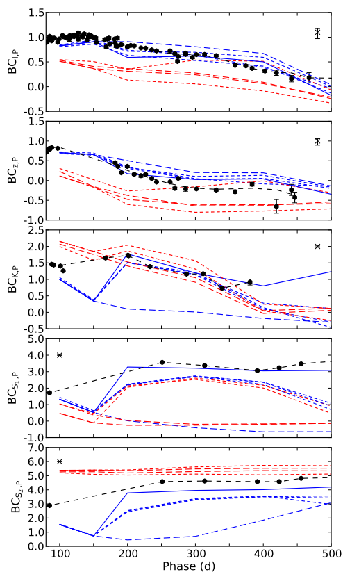
Fig. 20. The 100–500 days observed (black circles) and J14 model pseudo-BCs for the I , z , K , S_1 and S_2 bands. The model families differing in molecular cooling (complete; red, none; blue) and the optical depth of the dust (0; long-dashed, 0.25; short-dashed, 0.44; solid) are shown. 17 M_{\odot} and medium mixing models are not displayed. The error bars arising from the extinction are marked in the upper left or right corner.
