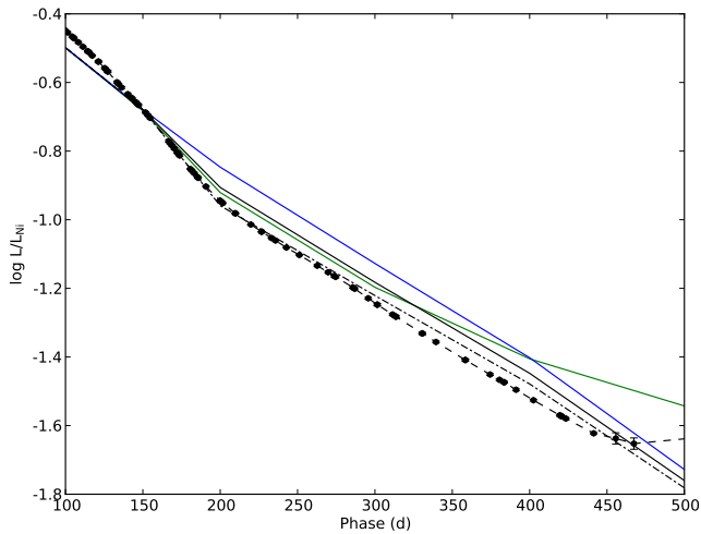
Fig. 19. 100-500 days observed (black circles) and J14 model optical pseudo-bolometric lightcurves normalized to the radioactive decay chain luminosity of 0.075 M_{\odot} of ^{56}\text{Ni} . The optimal model (12C; black solid line), the tweaked optimal model (12F; black dashed-dotted line) and model 12E (blue solid line), which only differ in the amount of dust, are shown together with model 12B (green solid line) which differ from the optimal model only in the positron trapping.
