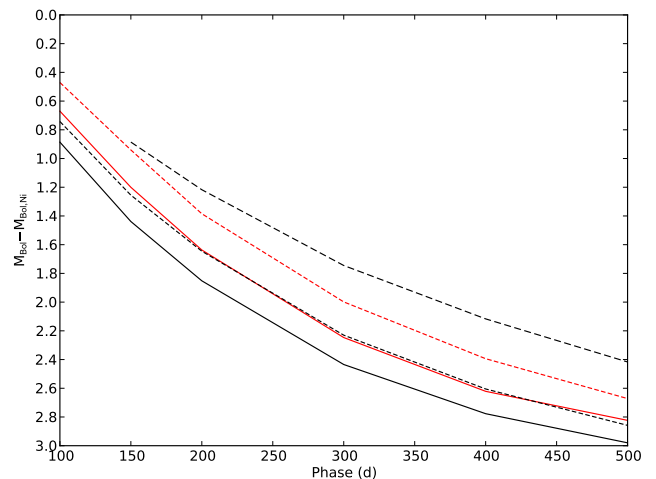
Fig. A.1. 100-500 days bolometric lightcurves for the J14 model normalized to the radioactive decay chain luminosity of 0.075 M_{\odot} of ^{56}\text{Ni} . The model families differing in initial mass and macroscopic mixing are displayed as follows: 12 M_{\odot} (solid lines), 13 M_{\odot} (short dashed lines), 17 M_{\odot} (long dashed lines), medium mixing (red), strong mixing (black).
