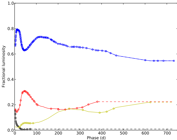
Fig. 7. Fractional UV (black dots), optical (blue dots) and NIR (red dots) and MIR (yellow dots) luminosity for SN 2011dh. Interpolations and extrapolations are displayed as solid and dashed lines, respectively.
