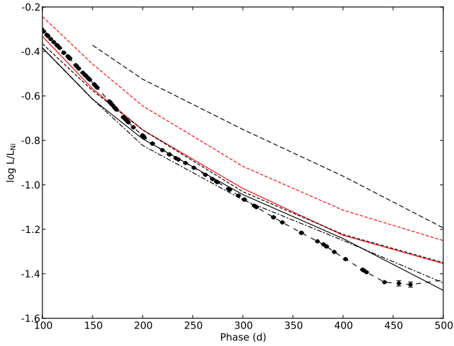
Fig. 18. 100-500 days observed (black circles) and J14 model optical to MIR pseudo-bolometric lightcurves normalized to the radioactive decay chain luminosity of 0.075 M_{\odot} of ^{56}\text{Ni} . Selected representatives (12A,12C,13A,13C,17A) of the model families differing in initial mass and macroscopic mixing are shown and displayed as follows: 12 M_{\odot} (solid lines), 13 M_{\odot} (short dashed lines), 17 M_{\odot} (long dashed lines), medium mixing (red), strong mixing (black). The tweaked optimal model (12F; black dashed-dotted line), which only differs from the optimal model (12C) in the properties of the dust, is also shown.
