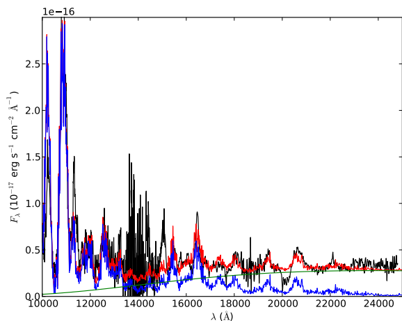
Fig. 25. Observed zJ and HK spectra at 198 and 206 days (black) compared to NIR spectra for the tweaked optimal model (12F; red) and model 12E (blue), which differ only in that \tau_{\text{dust}}=0 . The observed spectra were flux calibrated with the interpolated observed J , H and K magnitudes at 200 days and we also show the dust emission component for the tweaked optimal model (green).
