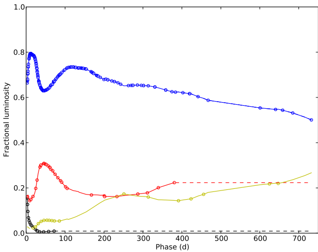
Fig. 7. Fractional UV (black dots), optical (blue dots), NIR (red dots) and MIR (yellow dots) luminosity for SN 2011dh. Interpolations and extrapolations are displayed as solid and dashed lines, respectively.
