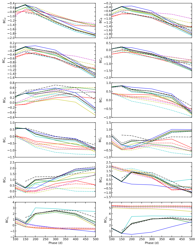
Fig. A.3. 100-500 days photometric BCs for the J14 models. The models are displayed as in Fig. A.2.
