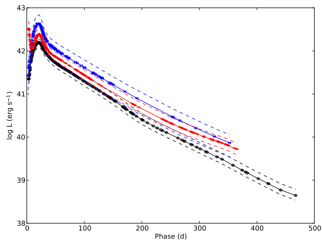
Fig. 5. Pseudo-bolometric optical to NIR lightcurve for SN 2011dh (black circles and solid line) calculated with the photometric method as compared to SNe 1993J (red crosses and solid line) and 2008ax (blue pluses and solid line). The upper and lower error bars for the systematic error arising from extinction and distance (dashed lines) are also shown.
