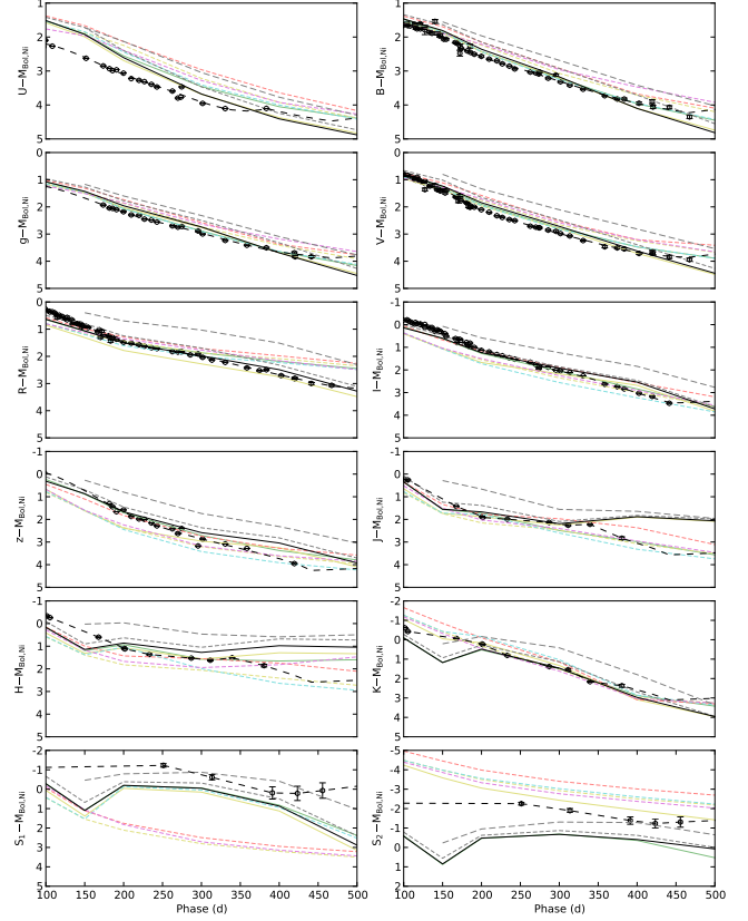
Fig. 19. 100-500 days J14 model and observed optical, NIR and MIR magnitudes normalized to the radioactive decay chain luminosity of 0.075 M_{\odot} of ^{56}\text{Ni} . Observations are displayed as black circles and the optimal model (12C) as a black solid line. The other models are displayed in shaded colour as in Fig. 18.
