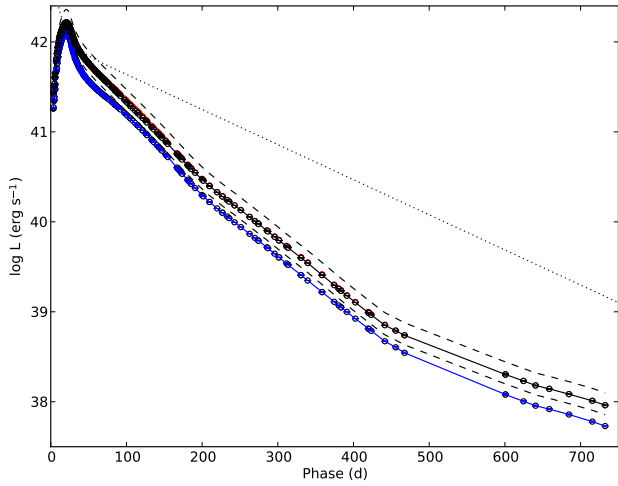
Fig. 6. Pseudo-bolometric UV to MIR (black) and optical (blue) lightcurves for SN 2011dh calculated with the combined spectroscopic and photometric methods (black circles and solid line). The upper and lower error bars for the systematic error arising from extinction and distance (black dashed lines) and the radioactive decay chain luminosity of 0.075 M_{\odot} of ^{56}\text{Ni} (black dotted line) are also shown.
