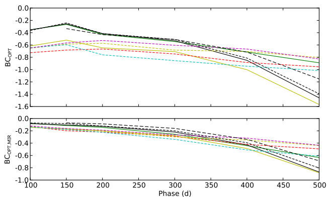
Fig. A.2. 100-500 days optical (upper panel) and optical to MIR (lower panel) BCs for the J14 models. The models are displayed as follows: 12B (green solid line), 12C (black solid line), 12D (yellow solid line), 13A (red short-dashed line), 13C (yellow short-dashed line), 13D (cyan short-dashed line), 13E (magenta short-dashed line), 13G (black short-dashed line), 17A (black long-dashed line).
