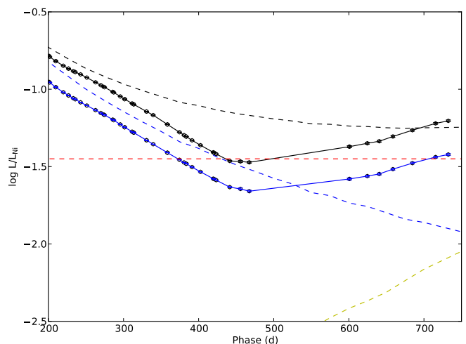
Fig. 23. Optical to MIR (black dots) and optical (blue dots) pseudo-bolometric lightcurves compared to the bolometric lightcurve (black dashed line), deposited ^{56}\text{Co} decay gamma-ray (blue dashed line) and positron (red dashed line) luminosity and deposited ^{57}\text{Co} decay luminosity (yellow dashed line) for the optimal steady-state NLTE model (12C). The lightcurves have been normalized to the radioactive decay chain luminosity of 0.075 M_{\odot} of ^{56}\text{Ni} .
