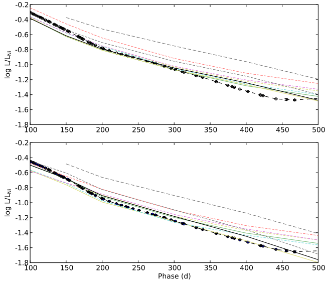
Fig. 18. 100-500 days J14 model and observed optical to MIR (upper panel) and optical (lower panel) pseudo-bolometric lightcurves normalized to the radioactive decay chain luminosity of 0.075 M_{\odot} of ^{56}\text{Ni} . Observations are displayed as black circles and the optimal model (12C) as a black solid line. The other models are display in shaded colour as follows: 12B (green solid line), 12D (yellow solid line), 13A (red short-dashed line), 13C (yellow short-dashed line), 13D (cyan short-dashed line), 13E (magenta short-dashed line), 13G (black short-dashed line), 17A (black long-dashed line).
