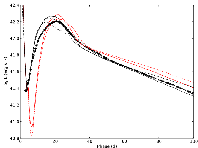
Fig. 20. 3-100 days bolometric lightcurves for the J14 model families differing in initial mass and macroscopic mixing calculated with HYDE as compared to the observed optical to MIR pseudo-bolometric lightcurve. The model families are displayed as follows: 12 M_{\odot} (solid lines), 13 M_{\odot} (short dashed lines), 17 M_{\odot} (long dashed lines), medium mixing (red), strong mixing (black).
