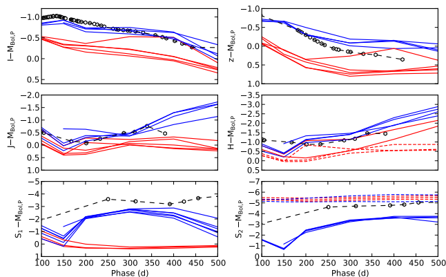
Fig. 21. 100-500 days model and observed M_{\text{Bol,P}} normalized I , z , J , H , S_1 and S_2 magnitudes. The I and z panels shows the no molecule cooling (blue) and molecule cooling (red) model families. The J and H band panels shows the local trapping (blue) and non-local trapping (red) model families and the H panel also shows the high contrast factor (solid lines) and low contrast factor (dashed lines) model families. The S_1 and S_2 panels shows the dust (blue) and no dust (red) model families and the S_2 panel also show the no molecule cooling (solid lines) and molecule cooling (dashed lines) model families.
