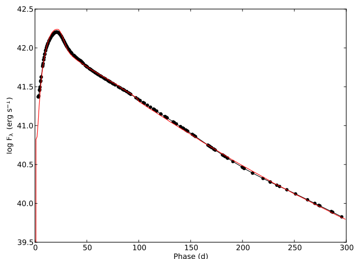
Fig. 26. Bolometric lightcurve for the optimal bare helium core model for SN 2011dh (red solid line) as compared to the observed U to 4.5 \mu\text{m} pseudo-bolometric lightcurve for the first 300 days (black dots and solid line). After 100 days the optimal bare helium core model flux has been multiplied with the fraction of bolometric flux within the U to 4.5 \mu\text{m} wavelength range for the optimal NLTE model.
